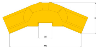
Internal 135°
