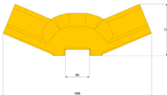
Internal 135°
